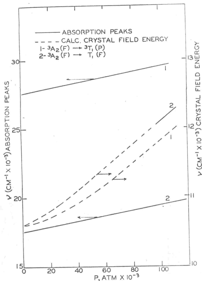
Fig. 12 Effect of pressure on d levels \text{Ni}^{++} in [\text{Ni}(\text{NH}_3)_6]\text{Cl}_2 .
